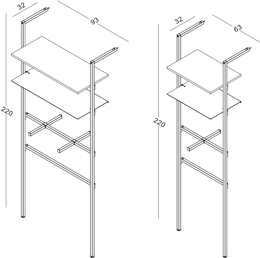
RBWSP2 appenderia frontale in metallo da applicare su RBWSP1-4 frontal hanging bar in metal to put on RBWSP1-4
